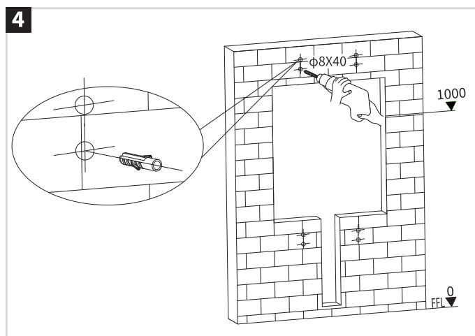
Drilling and installation of expansion screw
