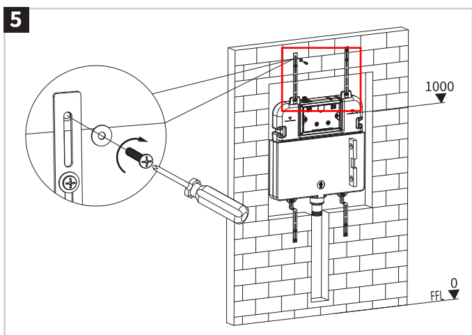
Installation of concealed cistern
