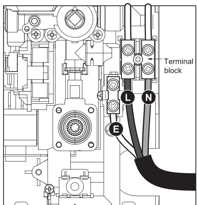
EXAMPLE - RIGHT SIDE ELECTRICAL CONNECTIONS
