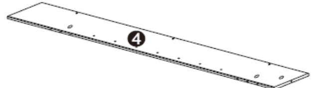
④x1 803x110x12mm
