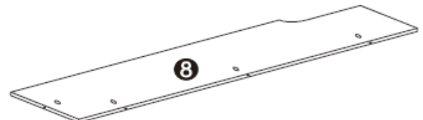
⑧x1 803x168x12mm
